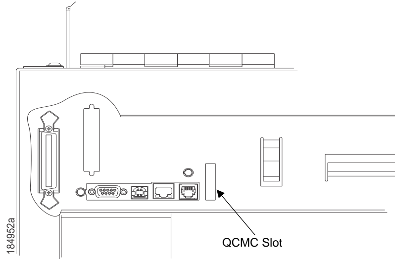
Figure 52 QCMC Slot on Back of Cabinet Model
