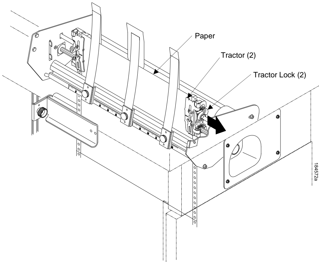
Figure 47 Adjusting the Horizontal Paper Tension
