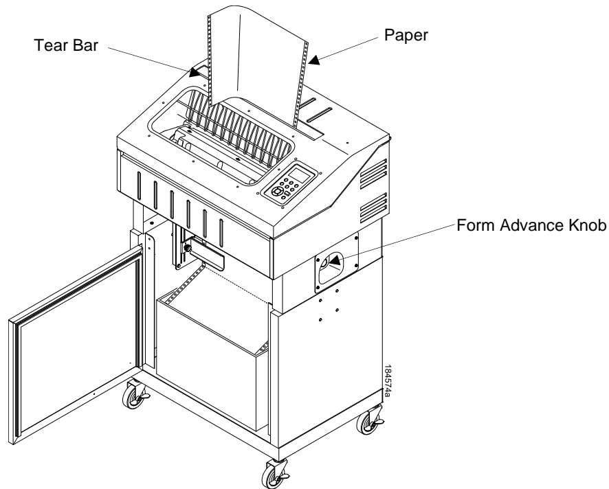
Figure 51 Setting The Tear Off Position
