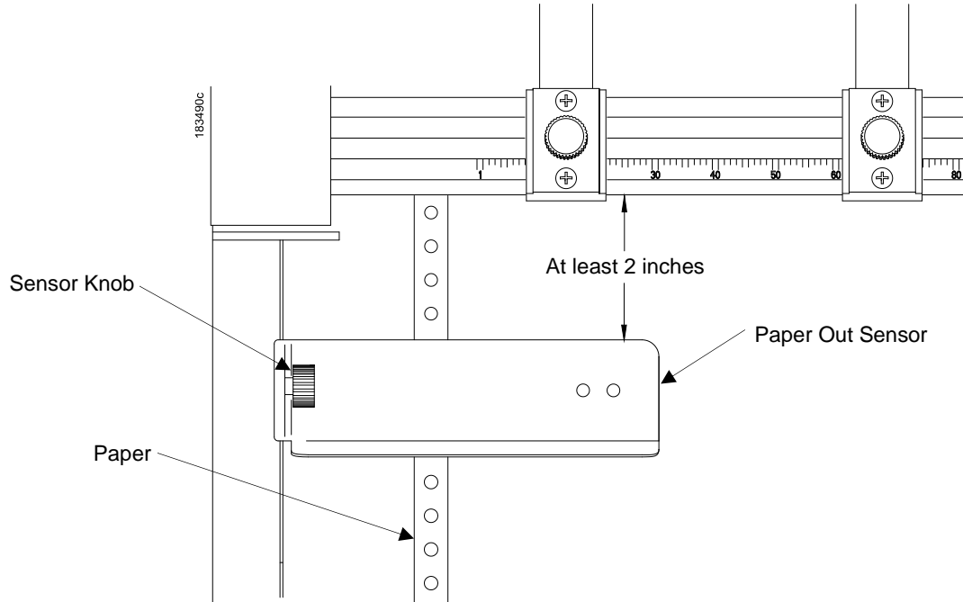
Figure 49 The Paper Out Sensor
