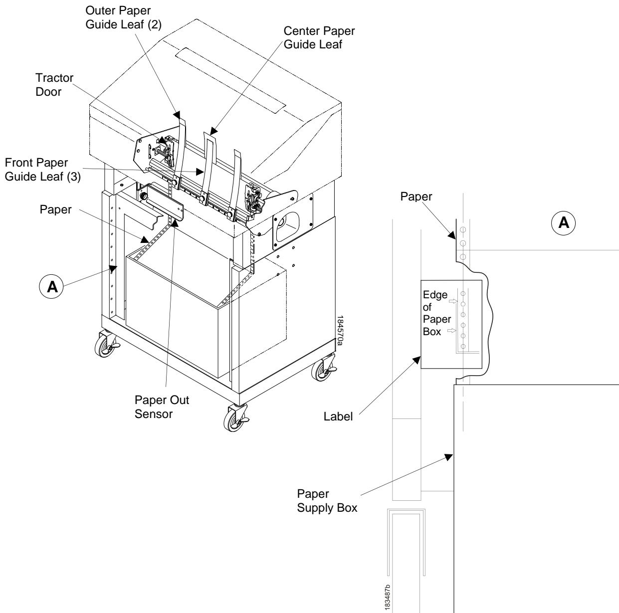
Figure 46 Loading Paper onto the Printer
