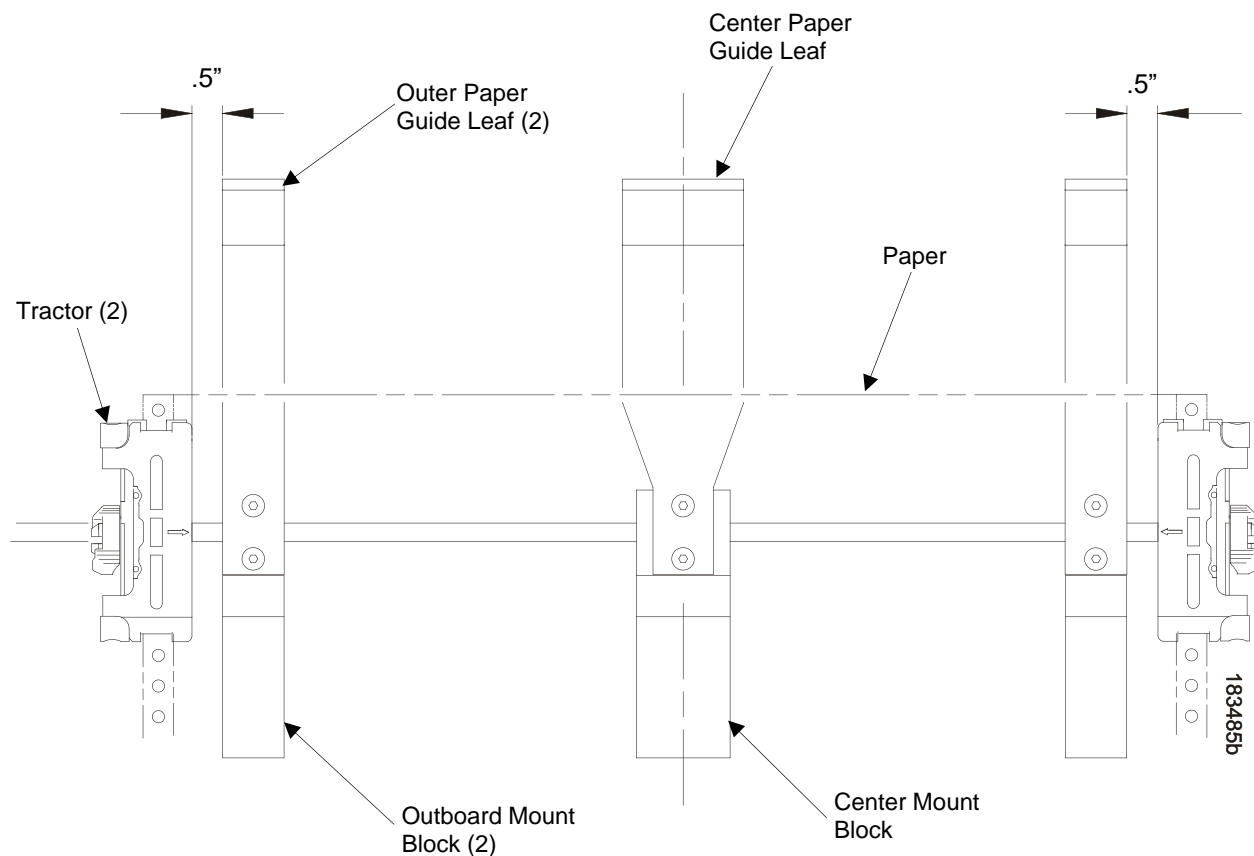
Figure 45 Adjusting Paper Guide Leaves
