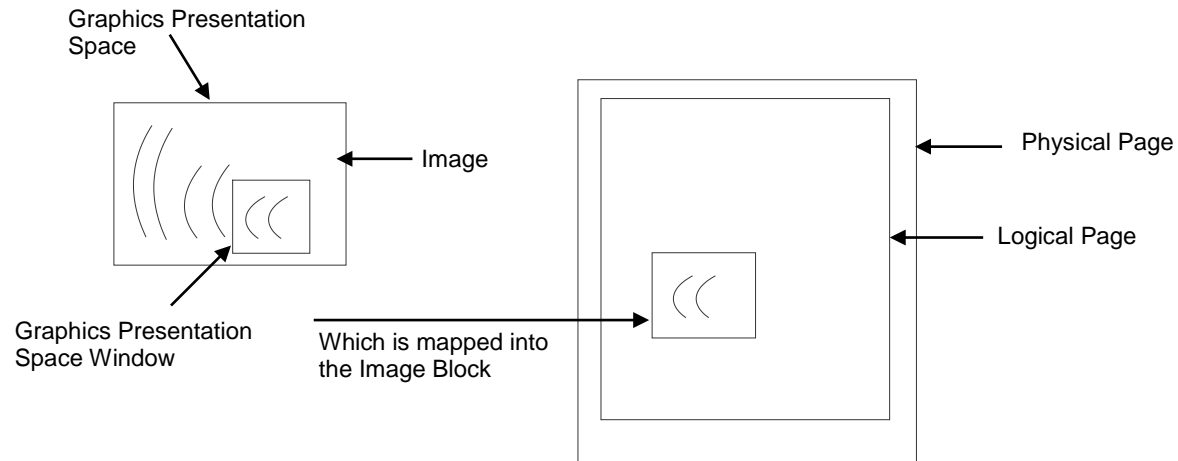
Figure 3 Generating Graphics
