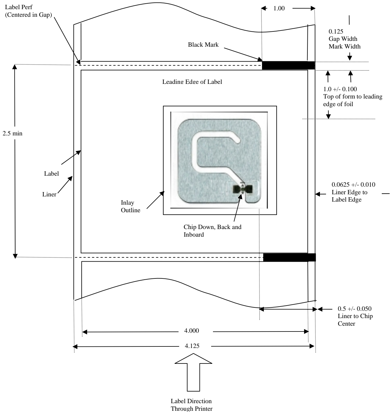
Printronix RFID Label Requirements for MP2 Avery AD812 G2 for 4in Wide x 2.5in Long (and Longer) Label
